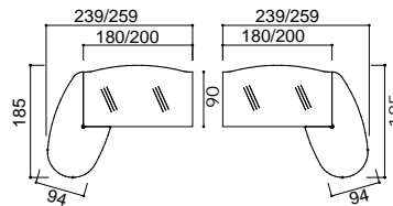
GLASS BOW FRONT DESK WITH EXTENSION lh/rh return
