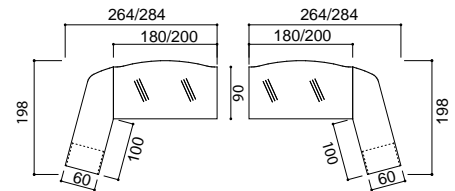
GLASS BOW FRONT DESK WITH RETURN AND PEDESTAL lh/rh return
