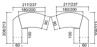
MELAMINE/GLASS CURVED DESK WITH RETURN AND PEDESTAL lh/rh return
