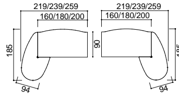
MELAMINE BOW FRONT DESK WITH EXTENSION lh/rh return
