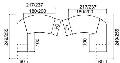
MELAMINE/GLASS CURVED DESK WITH RETURN AND MOBILE CABINET lh/rh return
